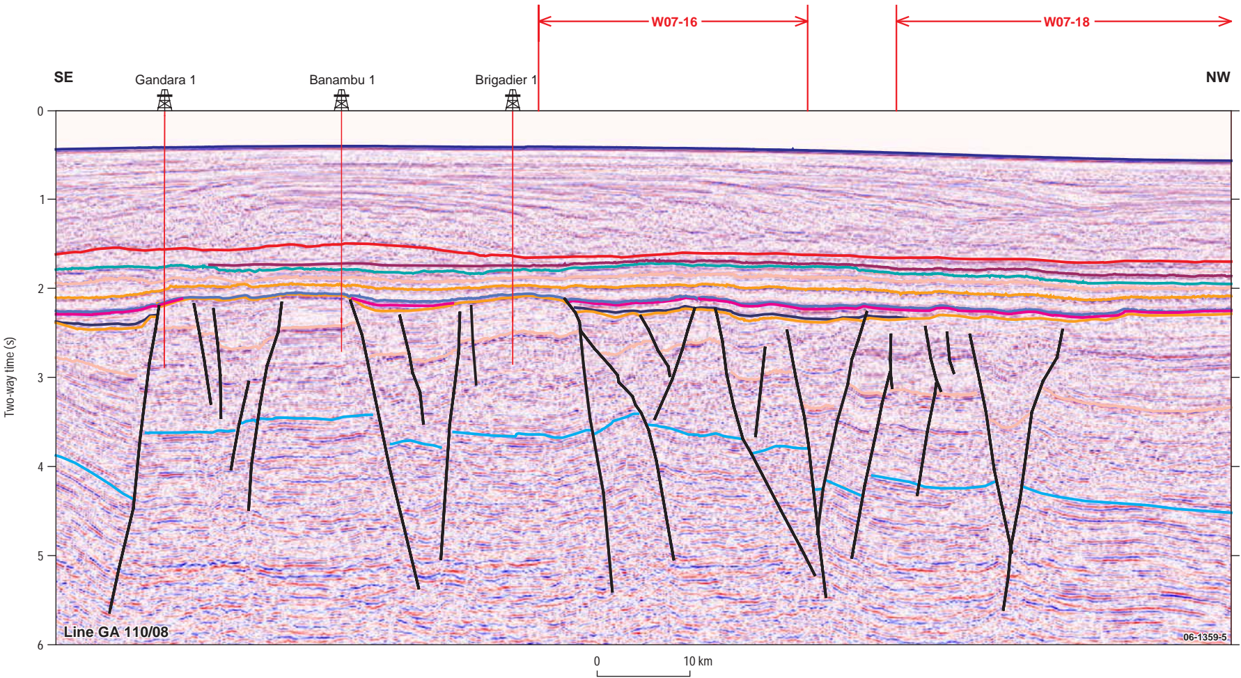
Figure 6. Regional seismic line 110-08, Northern Exmouth Plateau.
