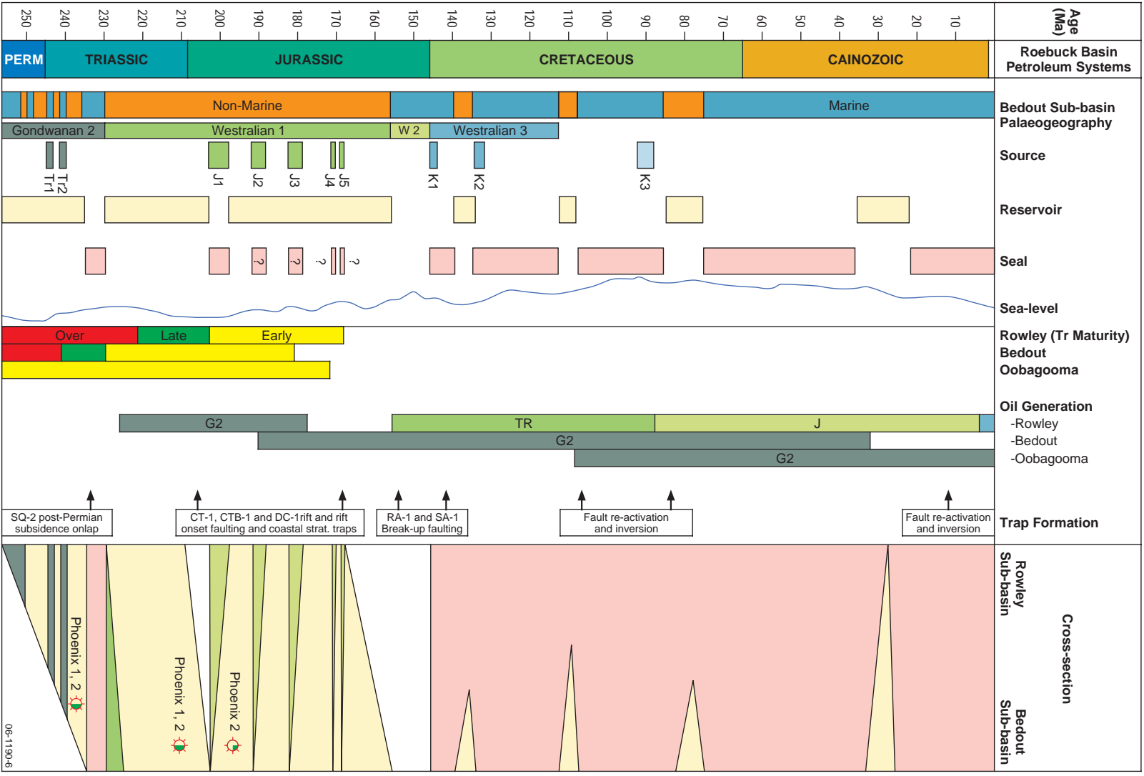
Figure 6. Petroleum systems of the Offshore Canning and Roebuck basins (after Smith, 1999 and Smith et al, 1999).
