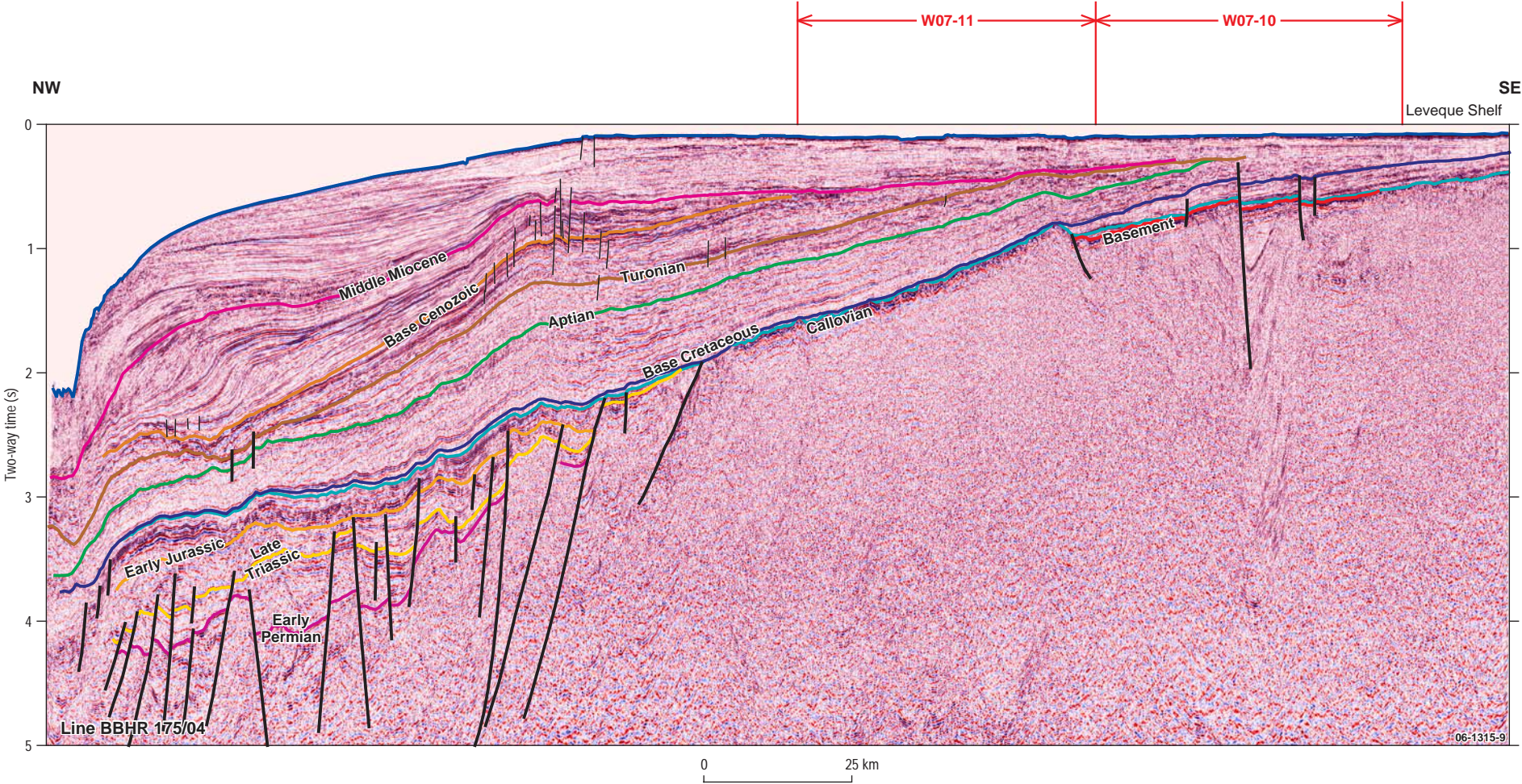
Figure 9. Seismic line BBHR 175/04 across areas W07-10 and W07-11 on the Leveque Shelf. Location of the line is shown in Figure 2. Regional seismic horizons are shown in Figure 3.
