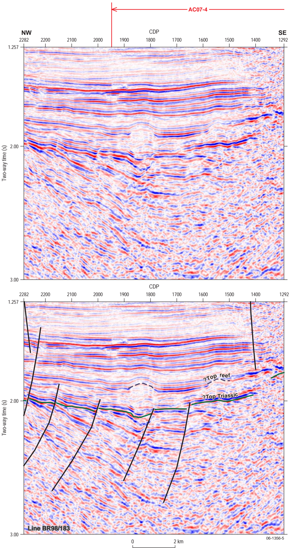
Figure 7. Seismic line BR98/183 highlighting potential top Triassic reefs or mound structures.
